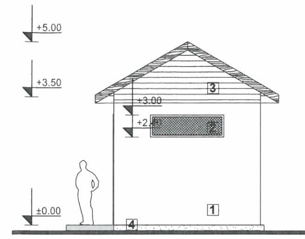
FATADA LATERALA scara 1:100
