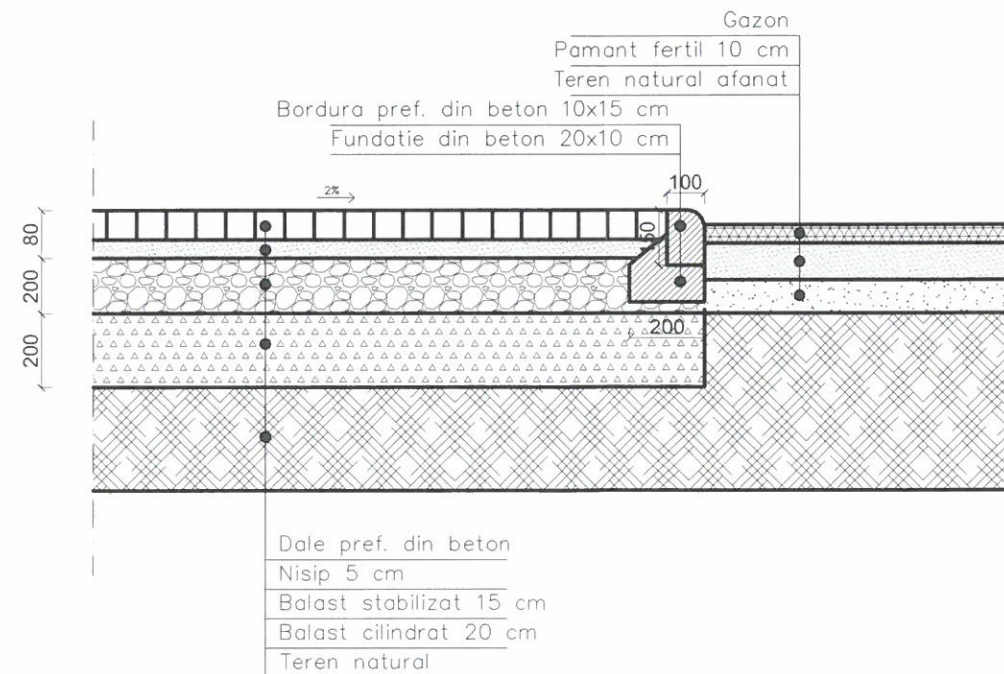
DETALIU – ALEE PIETONALA – SC. 1/20
