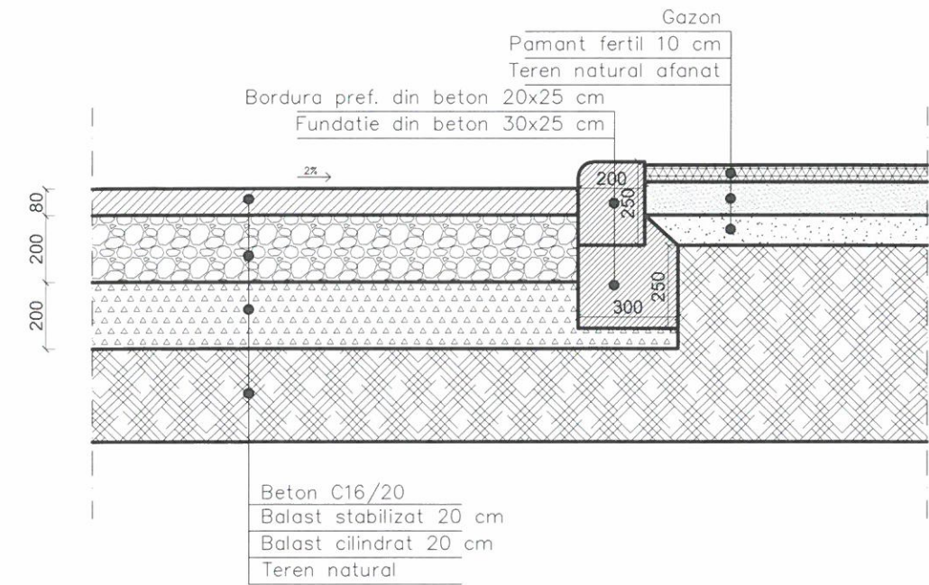
DETALIU – ALEE CAROSABILA – SC. 1/20
